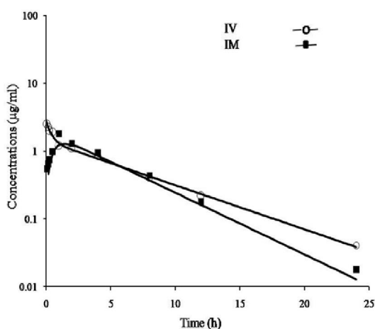
Figure 1. Semi-Logarithmic graph depicting the time-concentration of marbofloxacin in serum of buffaloes after a single IV (○) and IM (■) administration of 2 mg/kg b.wt. (n=5).
